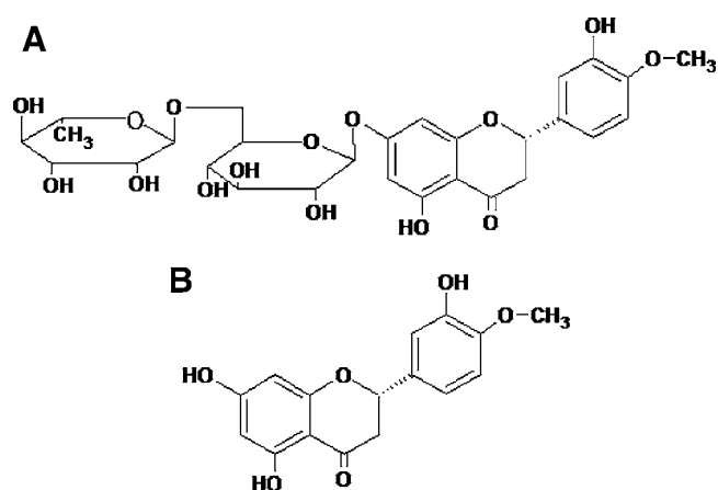
Fig. 1. A and B represents chemical structure of hesperidin (hesperetin—7-rhamnoglucoside) and hesperetin (3', 5,7-trihydroxy-4'-methoxy flavanone), respectively.
