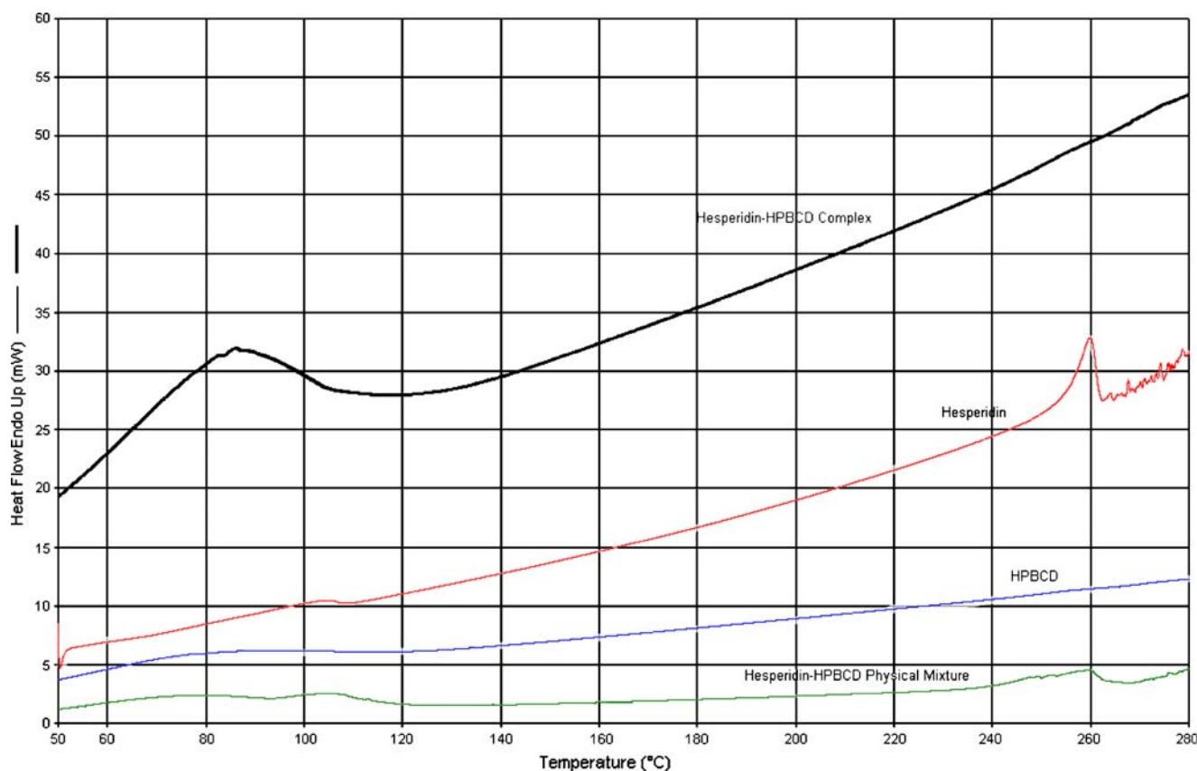
Fig. 5. DSC thermograms of the pure hesperidin and HP- \beta -CD, physical mixture of hesperidin and HP- \beta -CD (1:1 molar ratio) and the complex.
