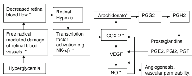
Fig. 2. Schematic representation of some of the currently identified pathways involved in the development and progression of diabetic retinopathy and macular degeneration. Asterisk indicates pathways which hesperidin and hesperetin can potentially inhibit.
