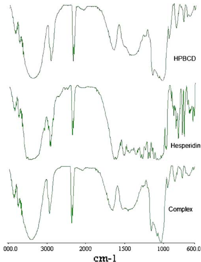
Fig. 6. FTIR spectra of the HP- \beta -CD, hesperidin and the complex.
